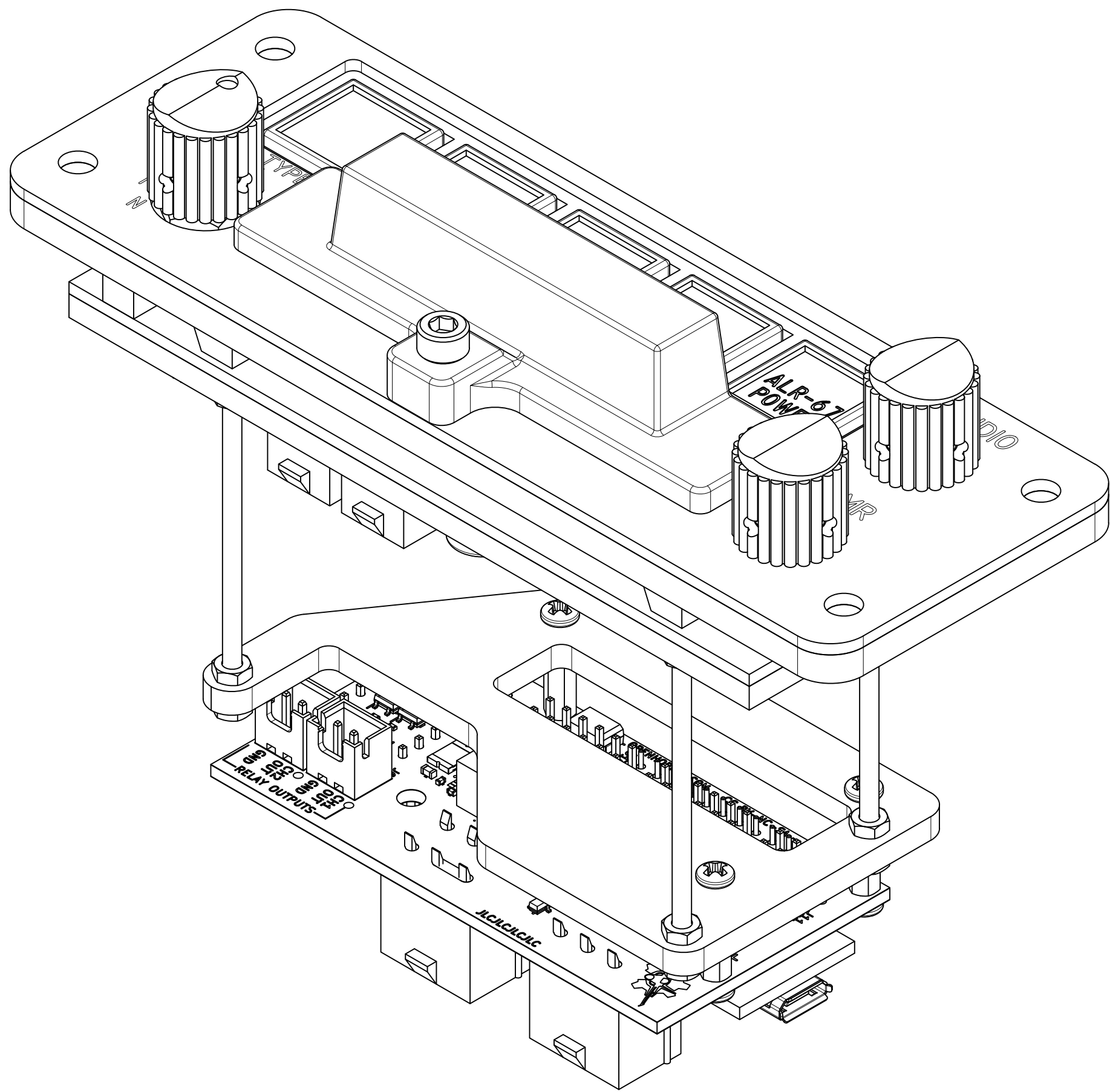
-1 ASSY SCALE 2:1
